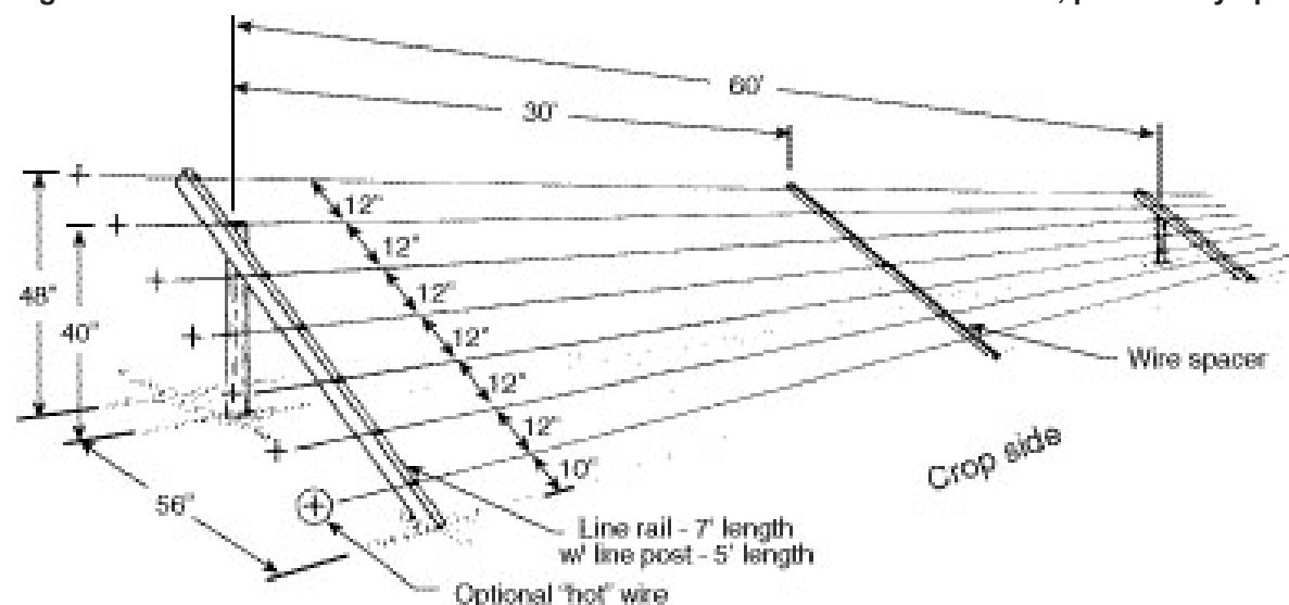
Figure 1. Electric 7-wire HT smooth wire slanted fence to control deer – wire, post & stay spacing
