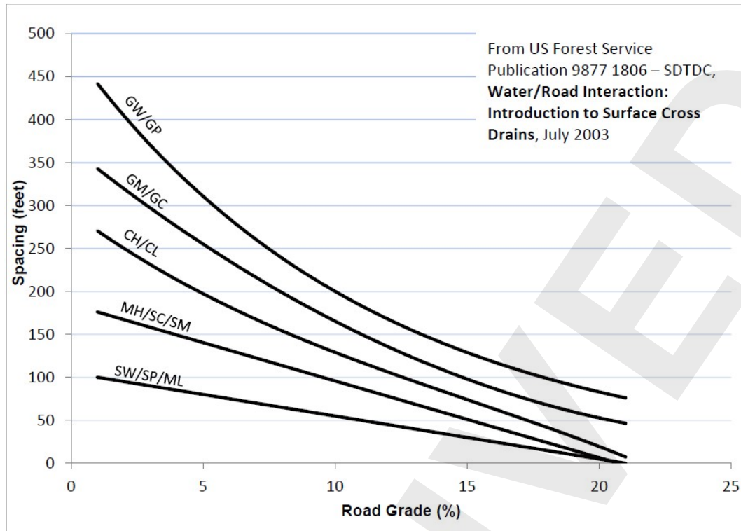
Figure 1. Recommended Spacing of Surface Cross Drains Based on Native Soil Types
