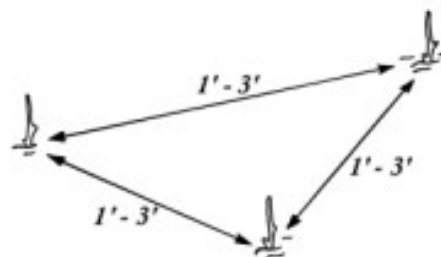
Figure 5 – Live Stake Installation
