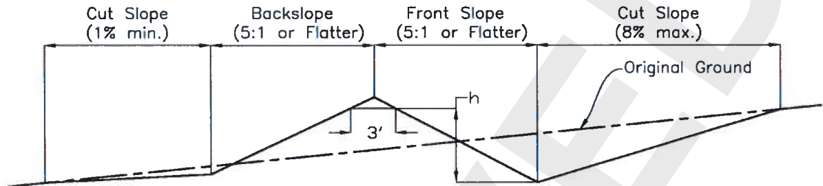
Figure 2. Broadbase Terrace Cross Section
