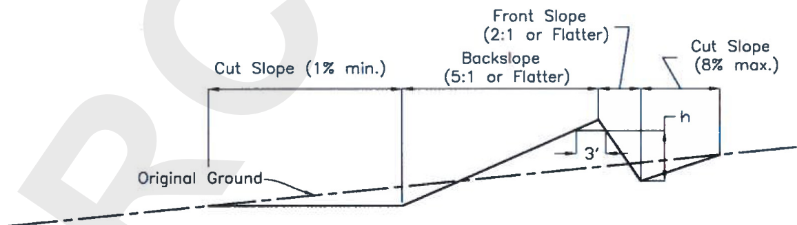
Figure 3. Grassed Front, Farmable Backslope Terrace Cross Section
