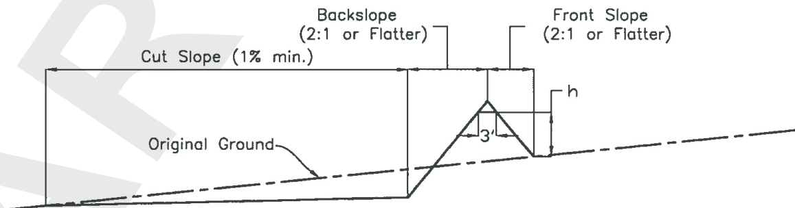
Figure 5. Narrow-Base Terrace Cross Section
