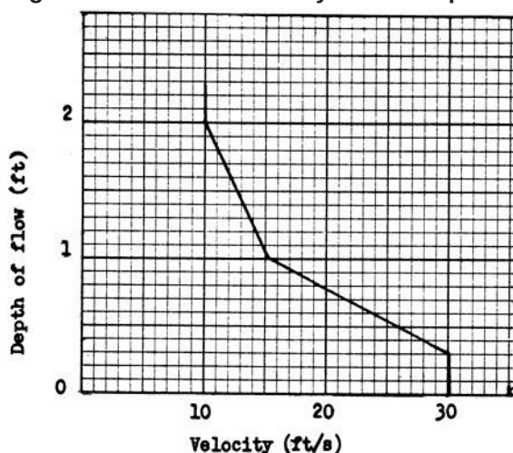
Figure 1. Maximum velocity versus depth of flow for concrete-lined channels
