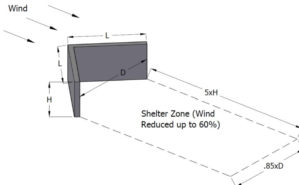
Figure 1. Snowdrift Protection from "V-shaped" Structures
