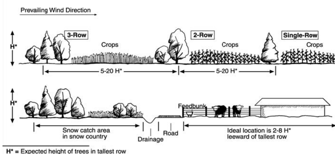
Figure 3: Examples of windbreaks used for crop protection and snow deposition
