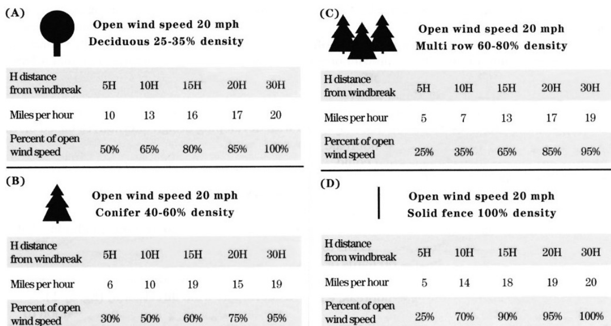
Figure 2: The density of the barrier affects the wind speed reduction leeward of the windbreak
