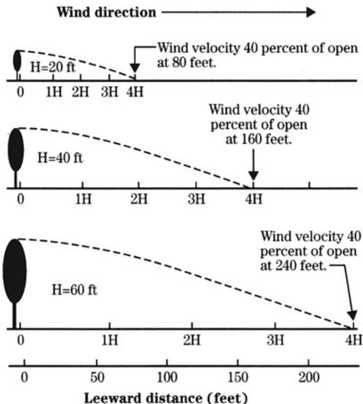
Figure 1: Wind protection is determined by barrier height
