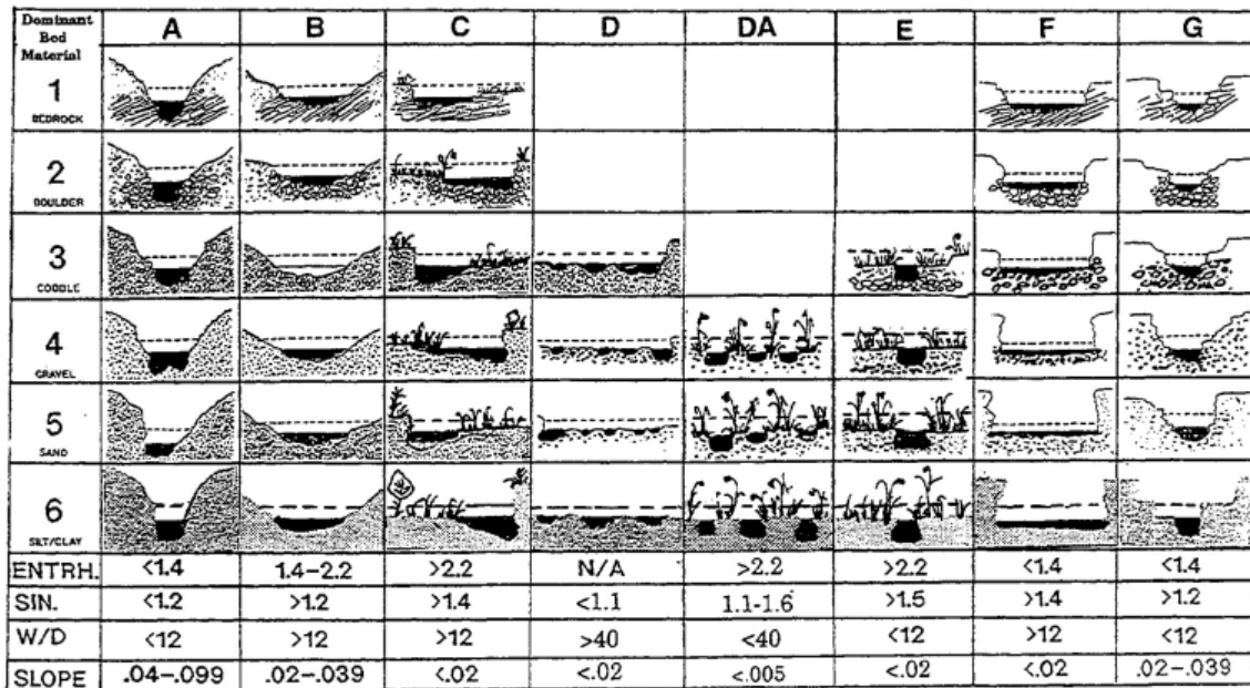
Fig. 4. Illustrative guide showing cross-sectional configuration, composition and delineative criteria of major stream types.
