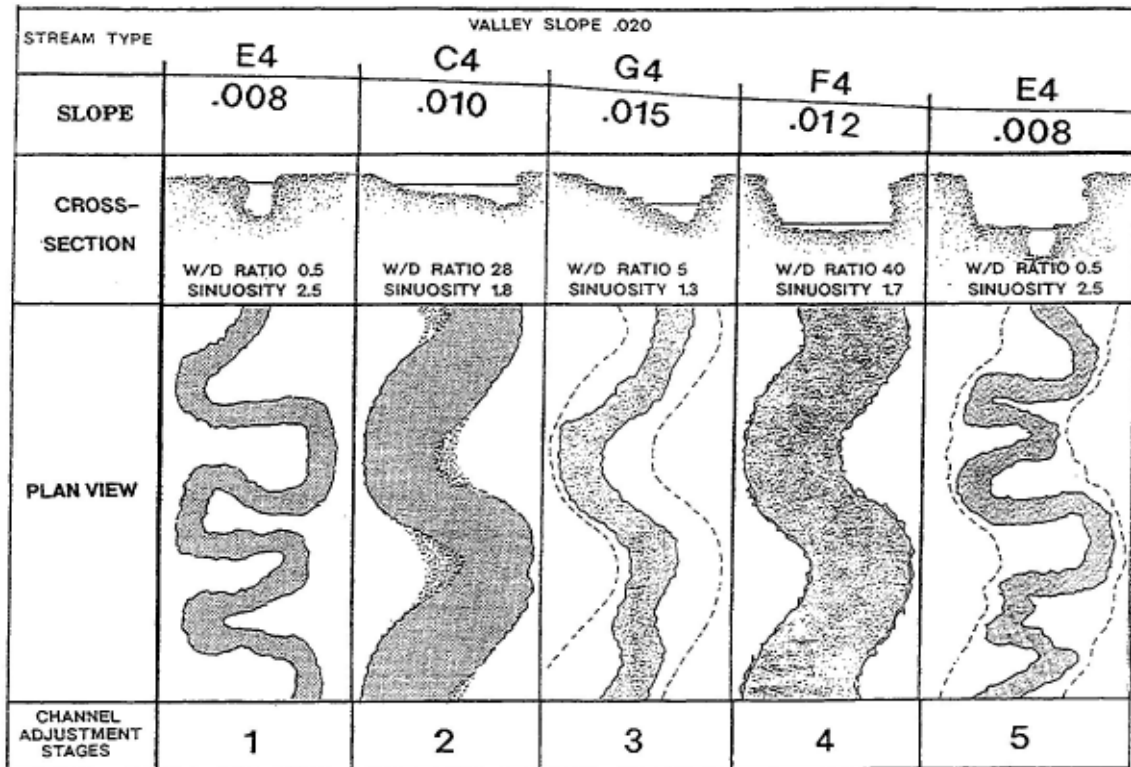
Fig. 9. Evolutionary stages of channel adjustment.
