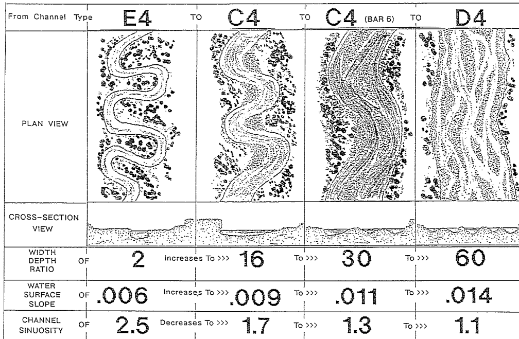
Fig. 8. Progressive stages of channel adjustment due to imposed stream bank instability.
