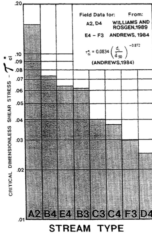
Fig. 13. Relationship of field verification of critical dimensionless shear stress values for various stream types.
