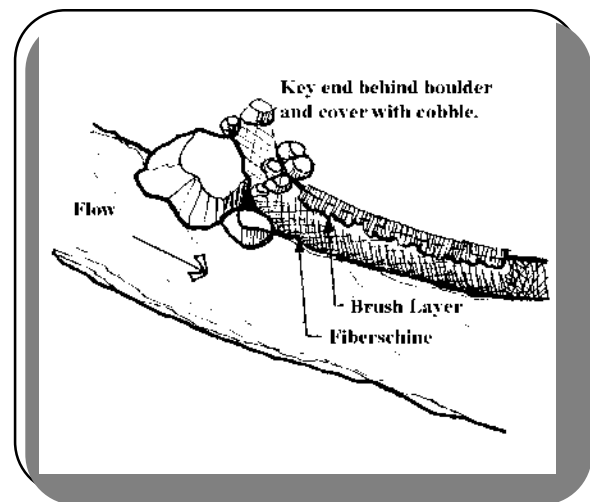
Fig. 3.8 Endpoint Protection
