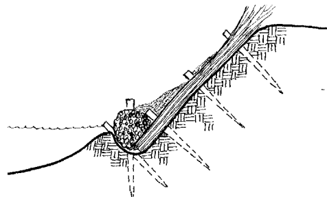
Step Six: Backfill
