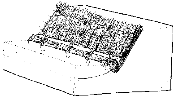
Brush Mattress
