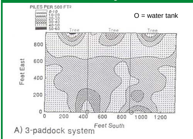
Figure 8. 3-Paddock System.
