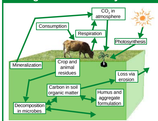
Figure 4. Carbon Cycle.
