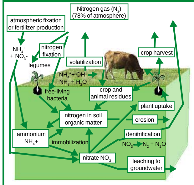
Figure 5. Nitrogen Cycle.
