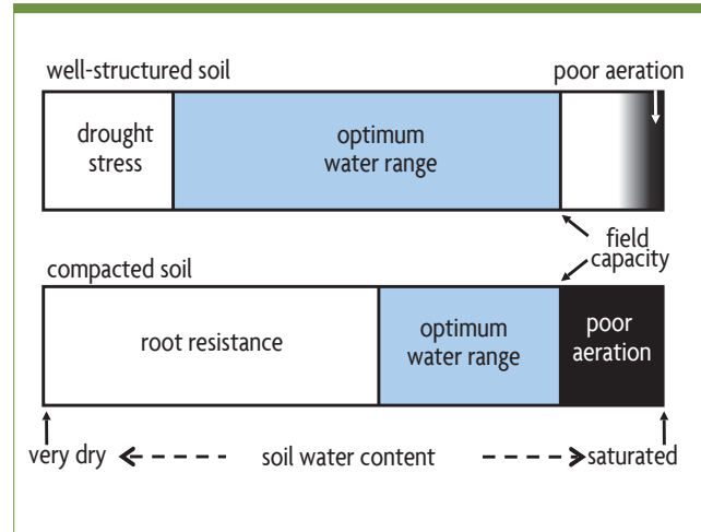
Figure 6.12. The optimum water range for crop growth for two different soils.
