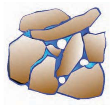
Figure 5.3. A moist sand with pores between grains that contain water and air. The larger pores have partially drained and allowed air entry, while the narrower ones are still filled with water.
