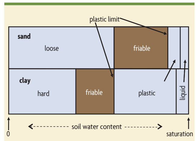
Figure 6.7. Soil consistency states for a sand and a clay soil (friable soil is best for tillage).
