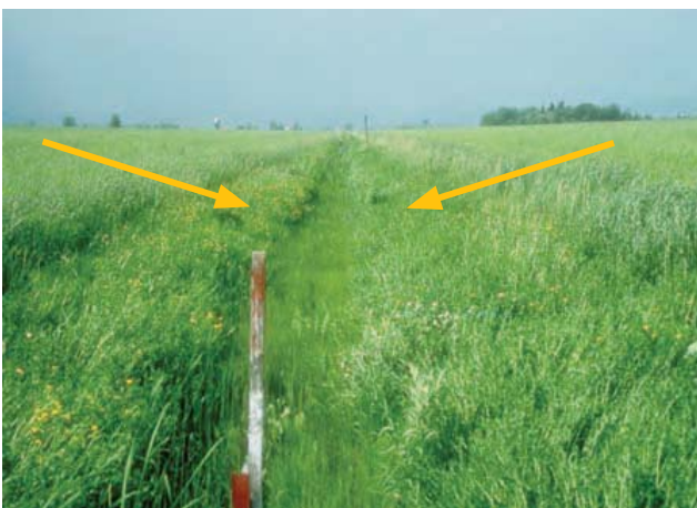
Figure 17.18. Surface drainage on clay soils in Ontario, Canada. Excess water travels over the surface to a grass waterway.
