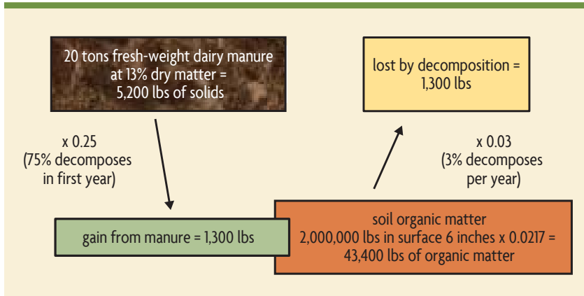
Figure 12.1. Example of dairy manure addition just balancing soil organic matter losses.
