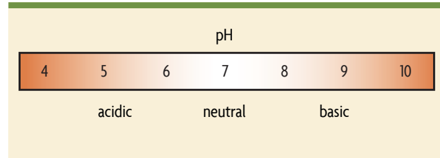
Figure 20.1. Soil pH and acid-base status.
