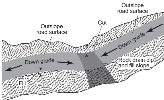
Figure 3-5. A drain dip sketch.
