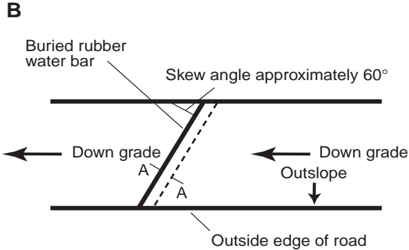
Figure 7-8. Installation specifications for rubber water bar.
